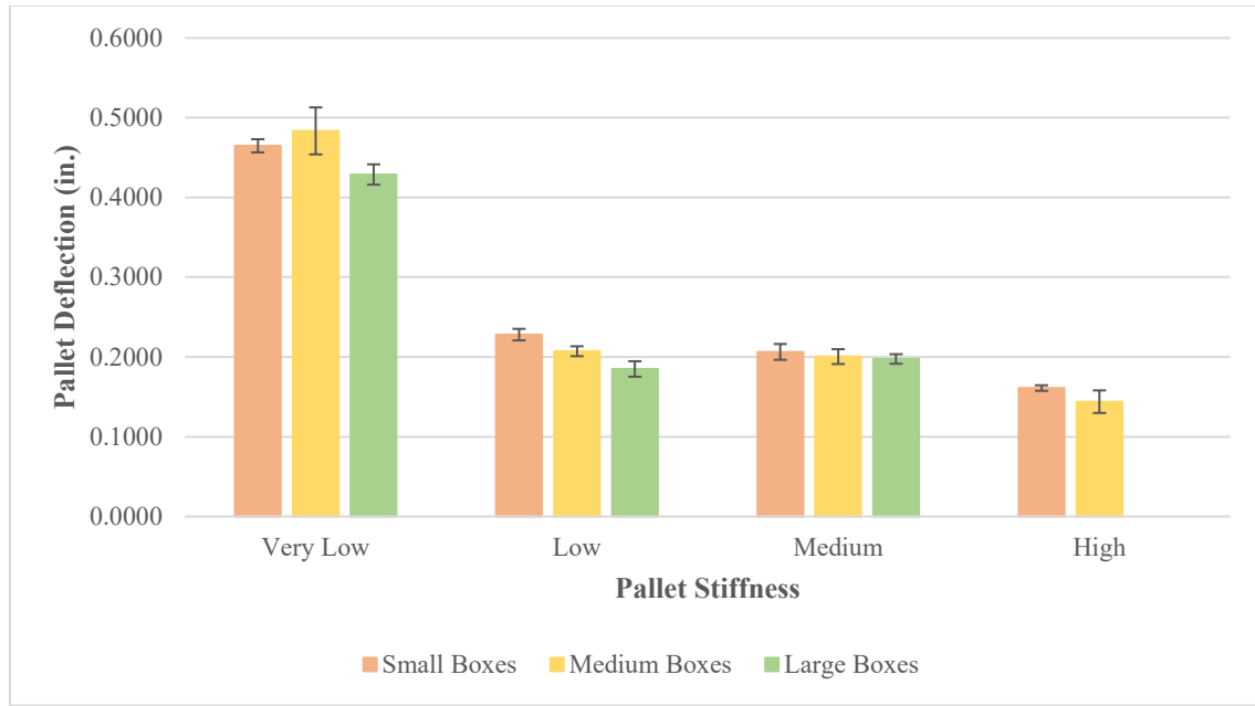
Figure 27: Average pallet center deflection during the warehouse racking across the width support condition using boxes with headspace. The whiskers represent standard deviation.
