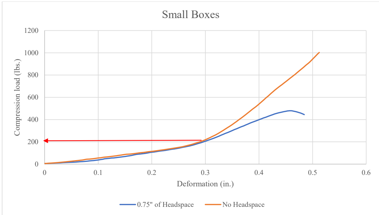
Figure 19: Load-deformation curve for small boxes with 0.75 inches of headspace and without headspace.
