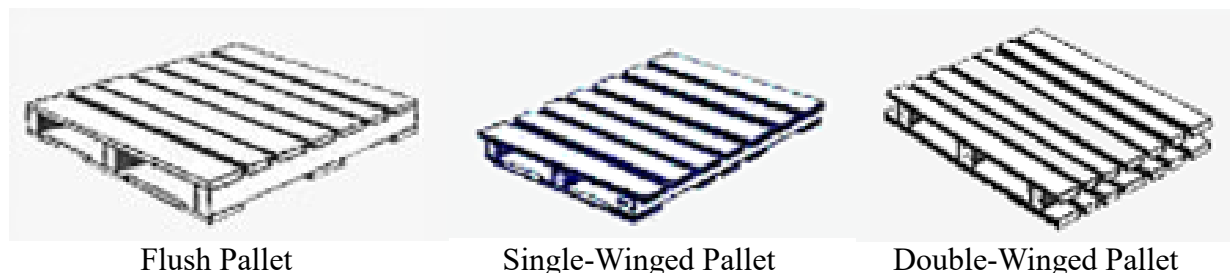
Figure 4: Examples of flush, single-winged, and double-winged stringer pallets (Adaptalift Group, 2013)
