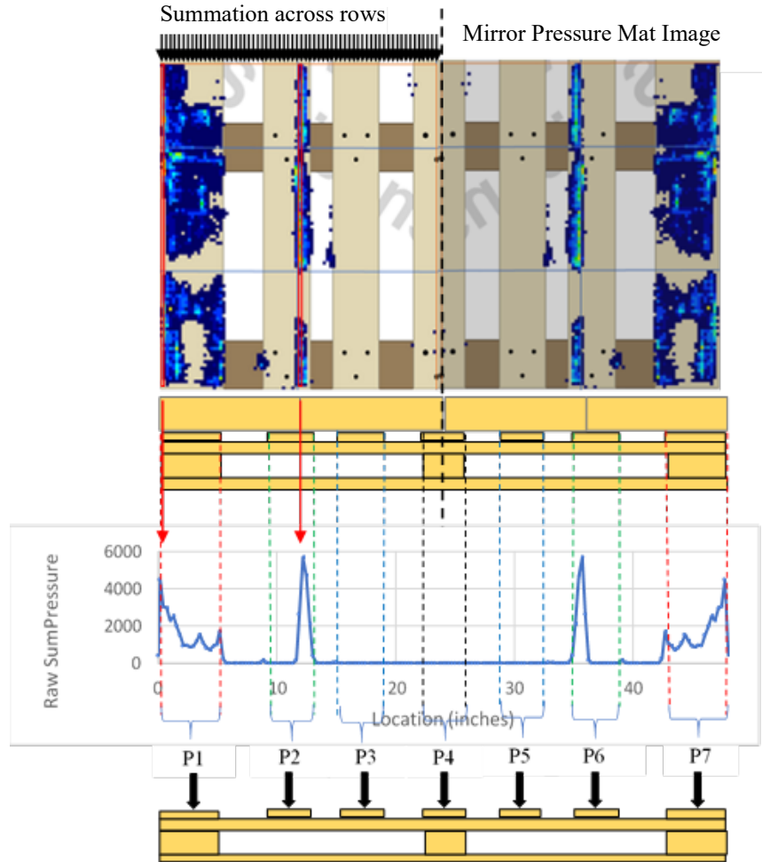
Figure 28: Visual representation of steps used for warehouse racking across the length (RAL) pressure mat analysis
